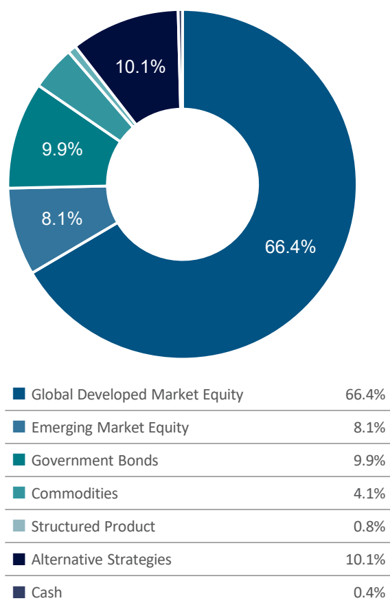
Figure 2: Asset Allocation
